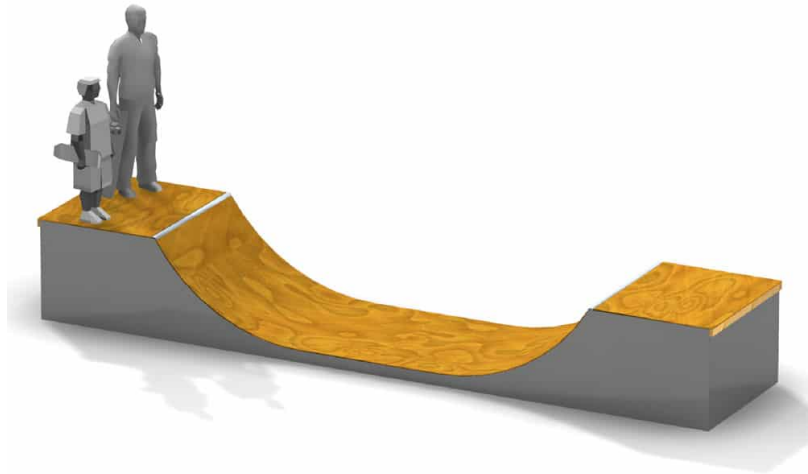
Wood Structure - Rampe Skate 1.5
